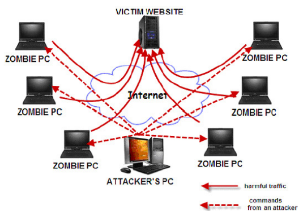
Figure 1: DDoS attack
